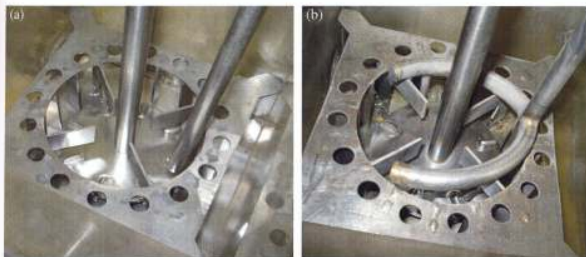
Figure 4.1: Impeller system of the Leeds cell used before (a) and after modification (b).
