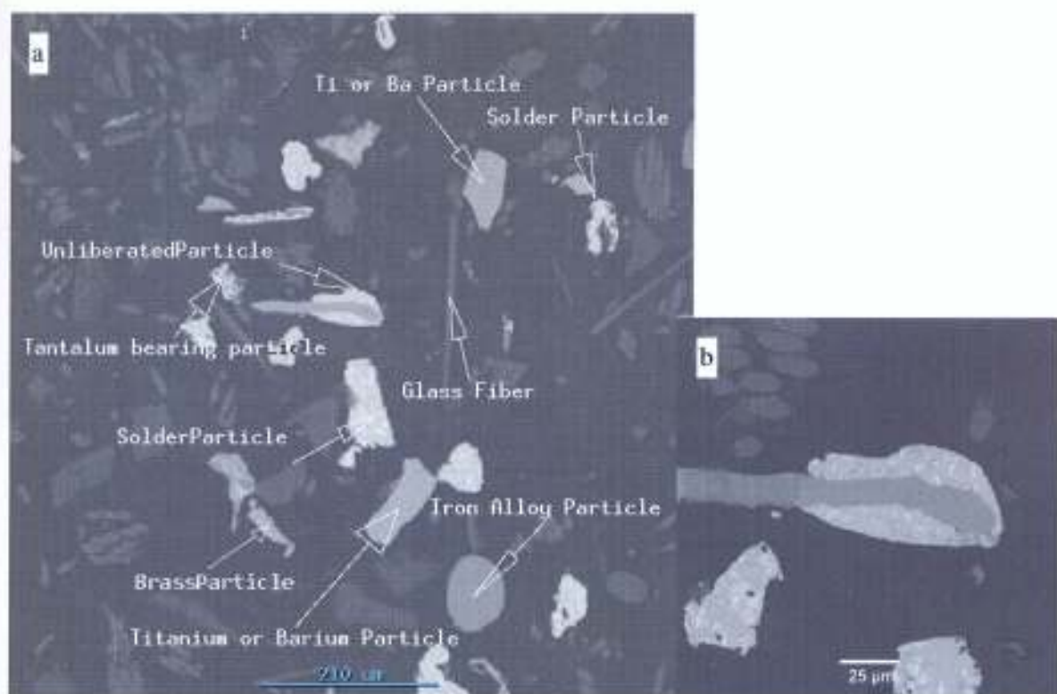
Figure 5.4: SEM back scattered electron images of -75+38\ \mu\text{m} printed circuit boards comminution fines section (a), and a close-up of an unliberated particle (b).
