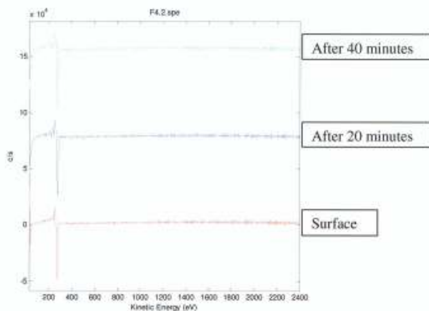
Figure A4.9: Comparison of AES survey spectra at various sputtering times on (indicative of depths from) the surface of fiber particle F4.
