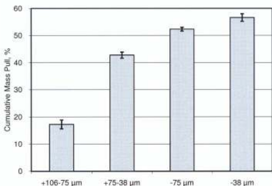
Figure 6.14: Cumulative mass pulls after 30 minutes for varying sample PSDs
