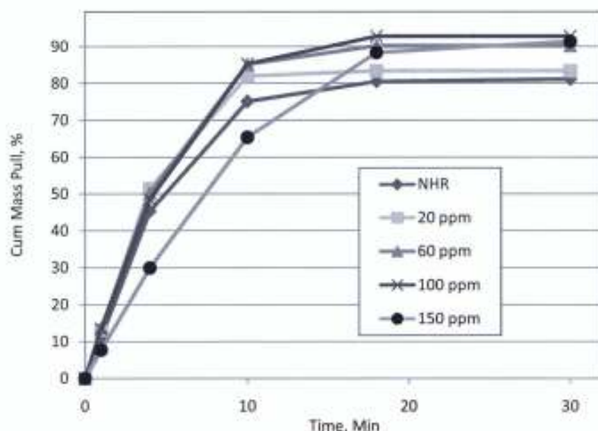
Figure 7.1: Mass pull over time in PBC comminution fine flotation with Betamin 127A as depressant at various dosages.
