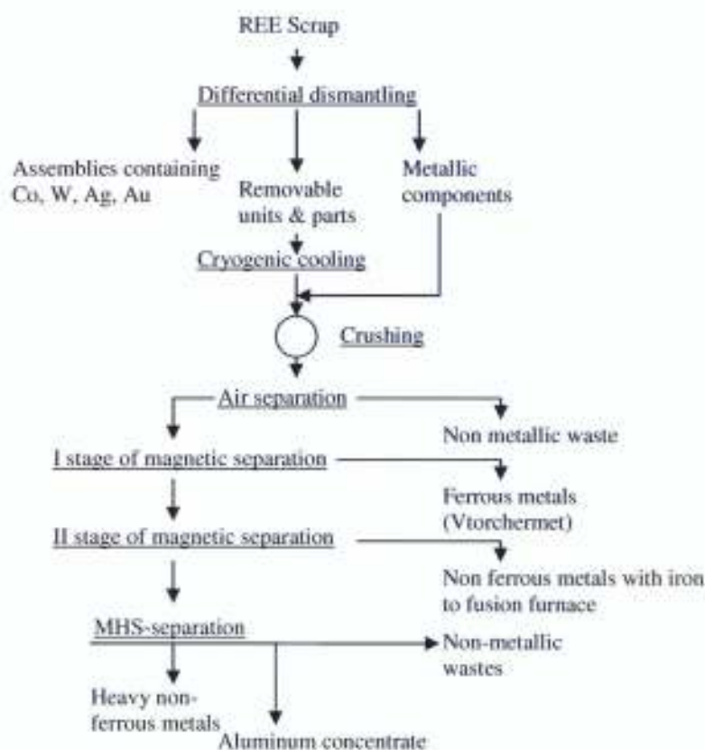
Figure 2.5: Flowsheet for reprocessing of multicomponent REE scrap (Kravchenko et al. , 1983 - Redrawn)
