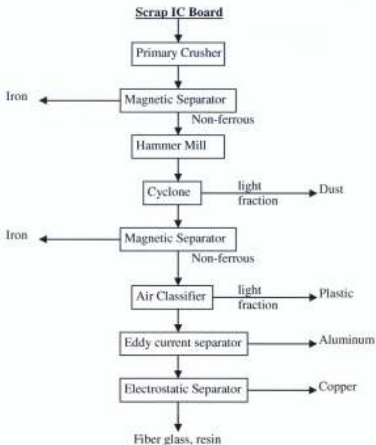
Figure 2.8: Huei-Chia-Dien Company's physical separation flowsheet for recycling of scrap IC boards (Lee et al. , 2004).
