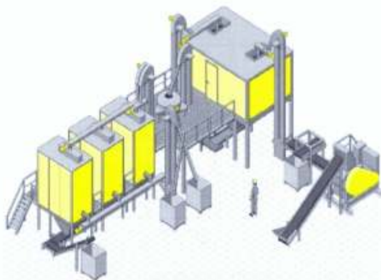
Figure 2.10: Hamos GmbH ERP – electronic recycling plant
